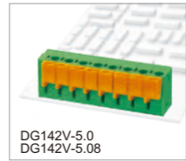
DG142V-7.62 450B/15A 0.2-1.5mm 2 300B/10A 22-16AWG Полосов 1P-XXP
