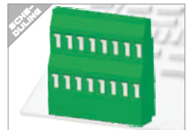
DG130AA-5.0 DG130AA-5.08 IEC 250B/20A 2.5mm 2 UL 300B/20A 26-12AWG Полосов 2*(2P,3P-24P)
